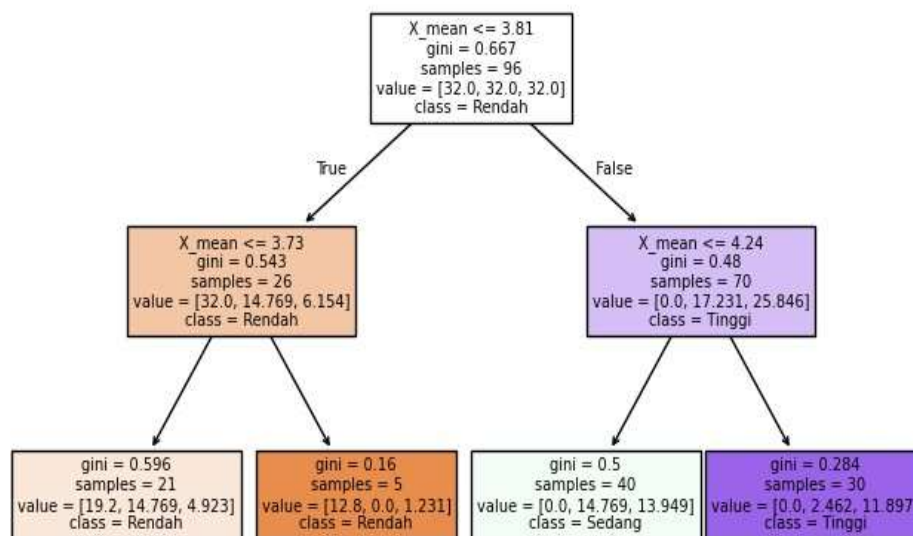
Figure 2. Decision Tree Model of Patient Satisfaction Prediction
